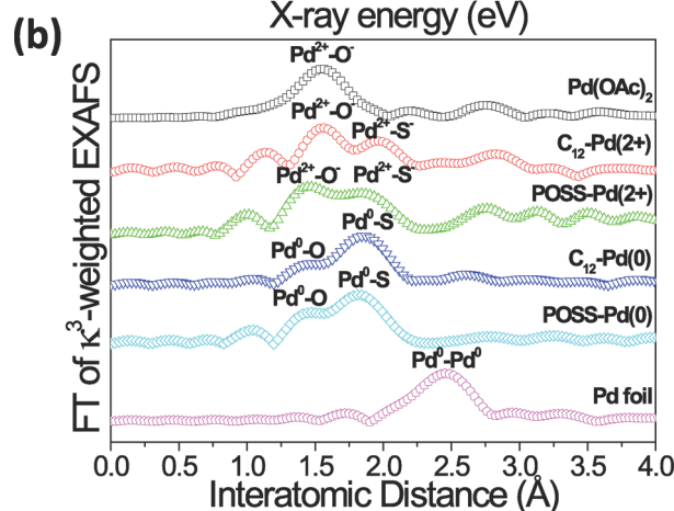
Figure 4. (a) Pd K-edge XANES spectra and (b) Fourier transforms of k^3 -weighted Pd K-edge EXAFS spectra of Pd(OAc) 2 , C 12 -Pd 2+ complexes, POSS-Pd 2+ complexes, C 12 -Pd(0) NPs, POSS-Pd(0) NPs, and standard Pd foil.
