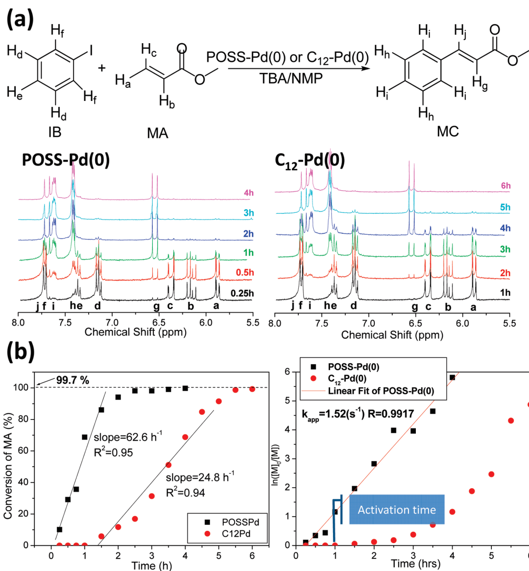
Figure 6. (A) 1 H NMR spectra of reaction mixture and (B) time–conversion and time–ln([M] 0 /[M]) profiles of Heck reactions using catalysts of POSS–Pd(0) and C 12 –Pd(0) NPs. Reaction conditions: 75 °C; catalysts, 0.1 g POSS–Pd(0) or 0.035 g C 12 –Pd(0) NPs (including 0.128 mmol Pd); NMP, 30 mL; iodobenzene and methyl acrylate, 5 mmol each; tributylamine, 7.5 mmol.
